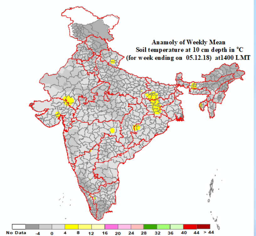
Anomaly
