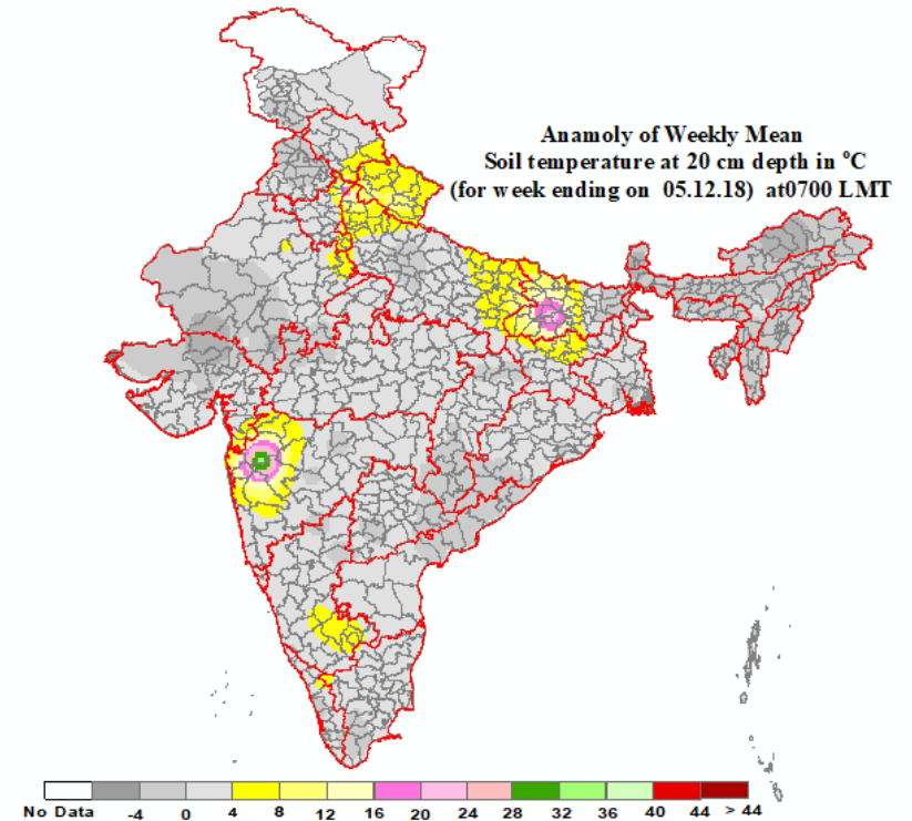
Anomaly
